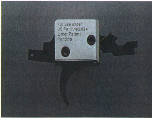
91501 AR15 Single Stage Curved small pin Trigger 91505 AR15 Single Stage Curved large pin Trigger
