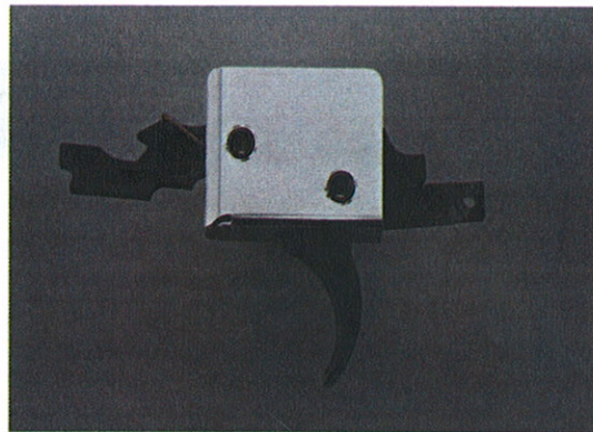
91501 AR15 Single Stage Curved small pin Trigger 91505 AR15 Single Stage Curved large pin Trigger
